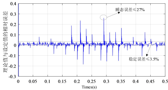
(b) 误差曲线
