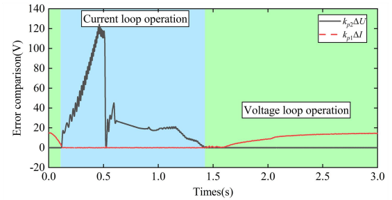
(c) 电压环与电流环误差曲线
