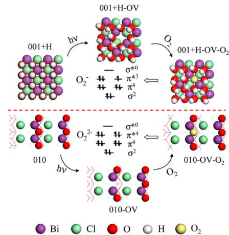
图3 BOC-001 和 BOC-010 表面拟议的分子氧活化过程 [21] Fig.3 Proposed molecular oxygen activation process on the surfaces of BOC-001 and BOC-010
