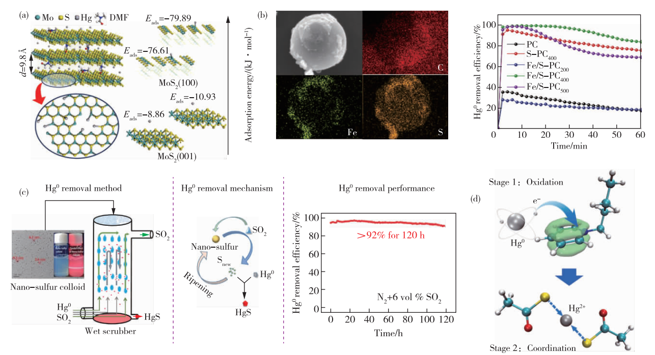
图 4 (a) DMF 插层 MoS 2 吸附剂 [13] ; (b) 碳载铁硫化物吸附剂 [16] ; (c) 纳米 S 液相捕汞剂 [17] ; (d) [Bpy][ThAc] 离子液体捕汞剂 [24] Fig. 4 (a) DMF-inserted MoS 2 adsorbent [13] ; (b) Carbon-supported iron sulfide adsorbent [16] ; (c) Nano S liquid mercury adsorbent [17] ; (d) [Bpy][ThAc] ionic liquid mercury adsorbent [24]
