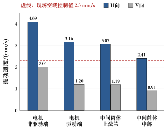
图 3 空载状态各测点 H/V 向振动速度实测值 Fig.3 Measured horizontal and vertical vibration velocities at the no-load test positions
