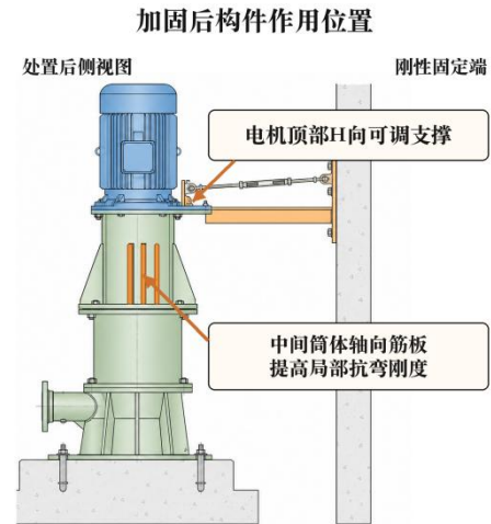
图 4 支撑加固方案示意 Fig.4 Support reinforcement scheme
